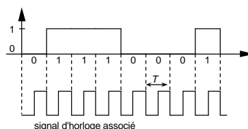
Transmission synchrone
